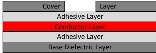
Single Sided Adhesive Based Stack Up
