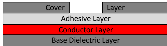
Single Sided Adhesive-less Stack Up
