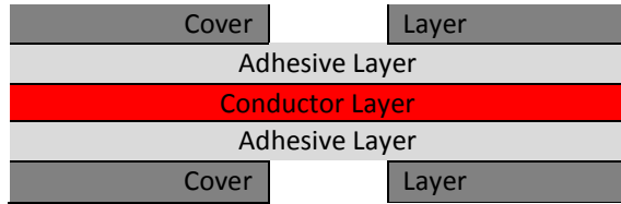
Single Sided Adhesive Based Stack Up
