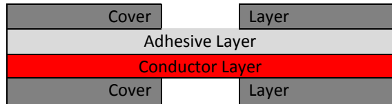
Single Sided Adhesive-less Stack Up
